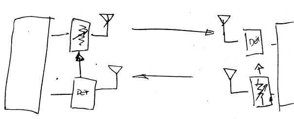
Figure 2 - Double ended Power Control - Open Loop
