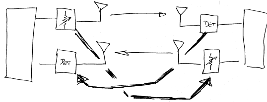
Figure 3 - Double Ended Power Control - Closed Loop
